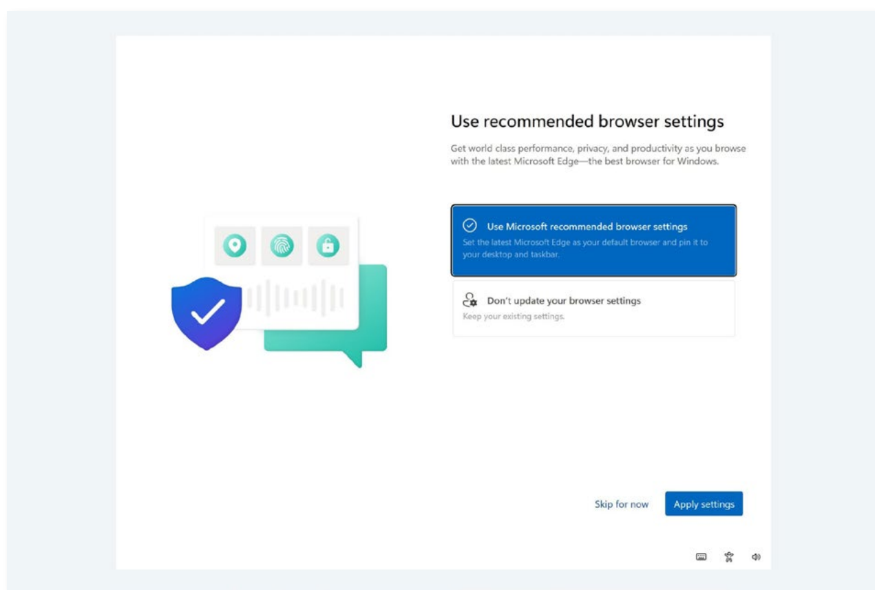
Figure 9: Windows 11 modal
